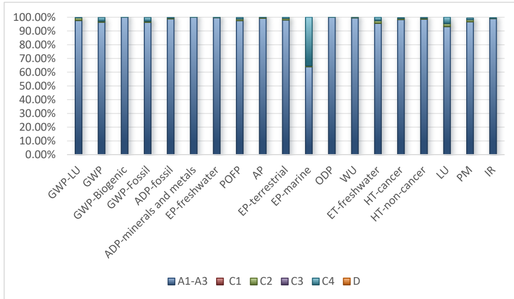
Figure 3. SoftenUp™ product each stage contribution to LCA results
