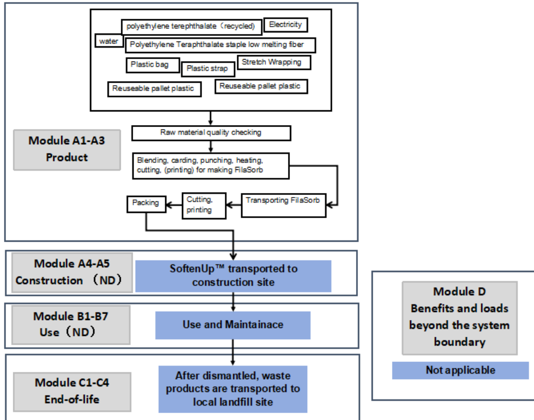
Figure 1. SoftenUp ™ Cradle to Gate System Boundary
